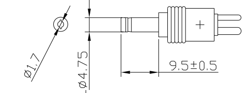
4. DETACHABLE PLUG. YELLOW PLASTIC RING HARDWARE. Ø1.7 X 4.75 X 9.5±0.5mm, I TYPE.
