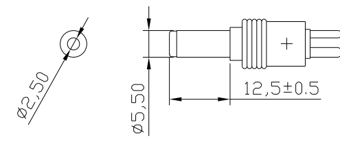
6. DETACHABLE PLUG. RED PLASTIC RING HARDWARE. Ø2.50 X 5.50 X 12.5±0.5mm, I TYPE.
