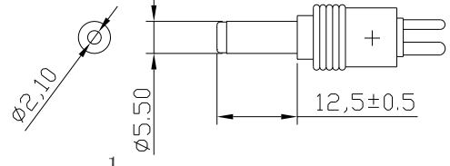
5. DETACHABLE PLUG. ORANGE PLASTIC RING HARDWARE. Ø2.10 X 5.5 X 12.5±0.5mm, I TYPE.
