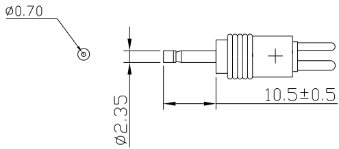
1. DETACHABLE PLUG. YELLOW PLASTIC RING HARDWARE. Ø2.35 X 0.7 X 10.5±0.5mm, I TYPE.
