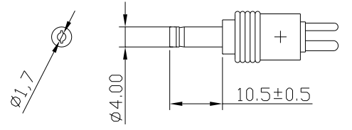
3. DETACHABLE PLUG. YELLOW PLASTIC RING HARDWARE. Ø1.7 X 4.0 X 10.5±0.5mm, I TYPE.
