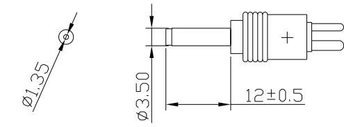
2. DETACHABLE PLUG. BLUE PLASTIC RING HARDWARE. Ø1.35 X 3.5 X 12±0.5mm, I TYPE.
